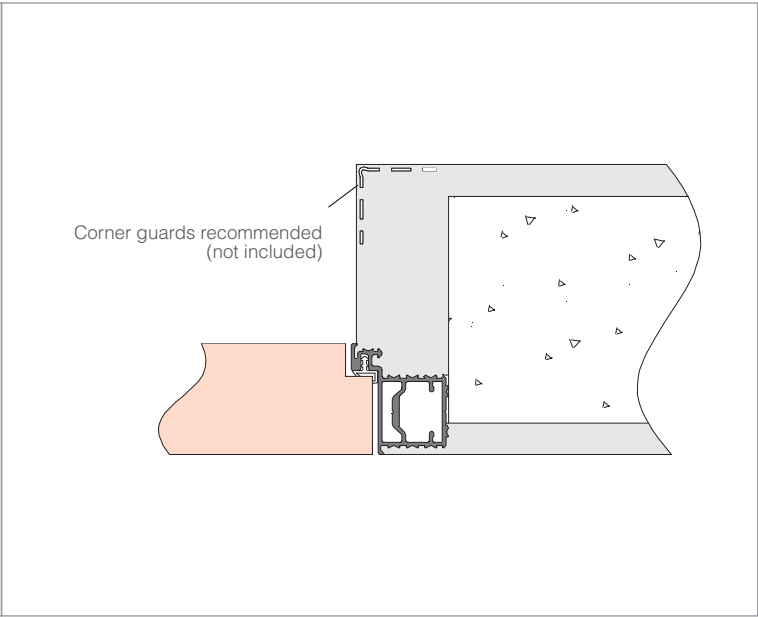
PULL OPENING
