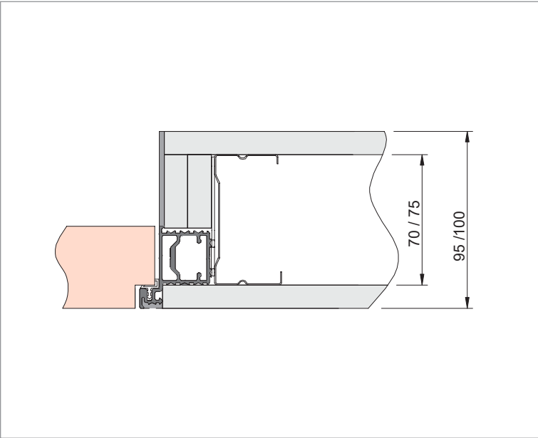
PUSH OPENING
